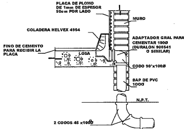
COLADERA PLUVIAL 4954 CLAVE: DBAP-01
