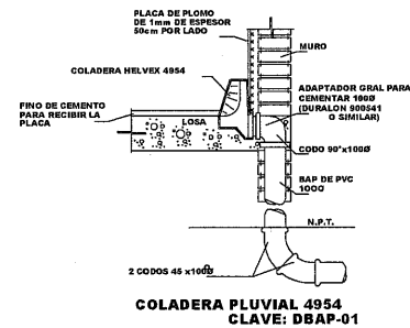
COLADERA PLUVIAL 4954 CLAVE: DBAP-01
