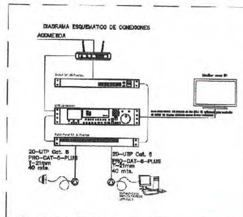
RACK IDF - GERIATRIA
