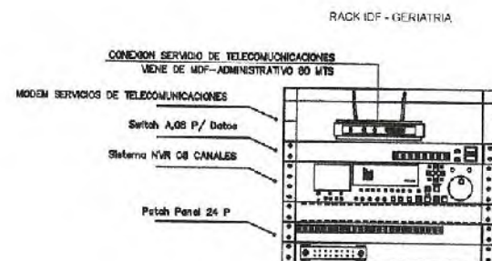
RACK IDF - GERIATRIA
